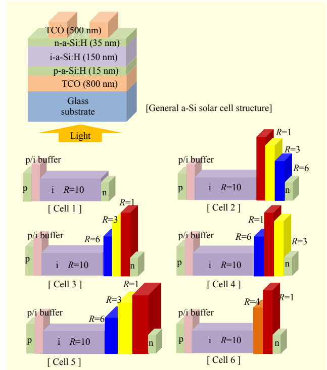
Fig. 1. Structures with various combinations of buffer layers at n/i interface in our experiments.
