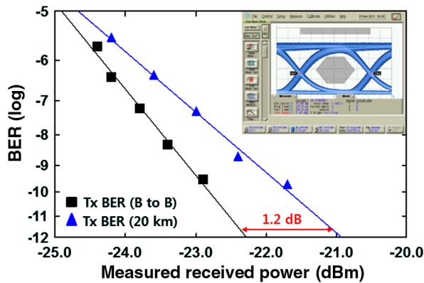
Fig. 2 The BER characteristic of the transmitter of the single TO-CAN BOSA at 1.25 Gb/s.
