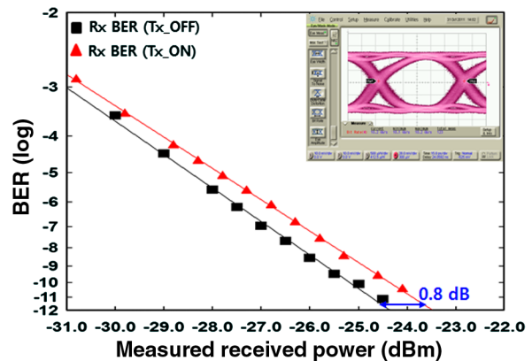
Fig. 3 Sensitivity test results of the receiver of the single TO-CAN BOSA at 10.3 Gb/s.
