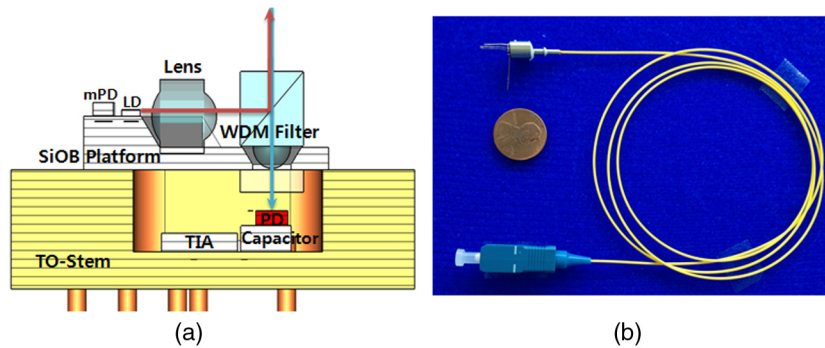
Fig. 1 Images of the proposed single TO-CAN BOSA. (a) Structure and optical signal path of the proposed single TO-CAN BOSA; (b) manufactured Single TO-CAN BOSA.
