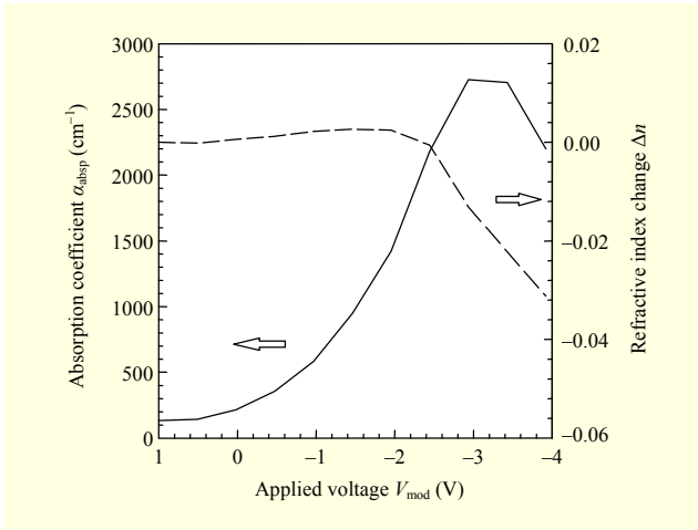
Fig. 3. Absorption coefficient and refractive index change as function of applied voltage of EA-MOD.
