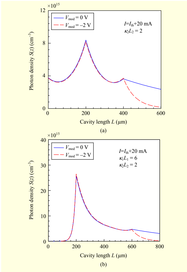
Fig. 5. Distributions of photon densities for (a) DFB-LD/EA-MOD and (b) DR-LD/EA-MOD during on-state and off-state.
