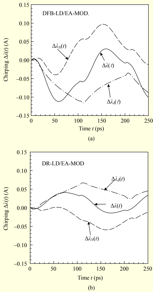
Fig. 10. Chirp and its components of (a) DFB-LD/EA-MOD and (b) DR-LD/EA-MOD. In this simulation, \kappa_2 L_2 = 2 and R_f = 0.01\% .
