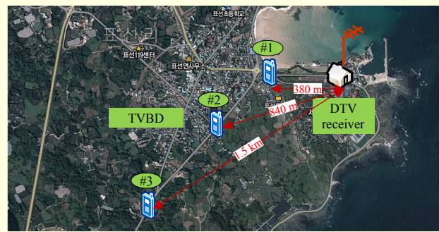
Fig. 11. Field test for required separation distance verification of 100 mW portable TVBDs in rural area near beach.
