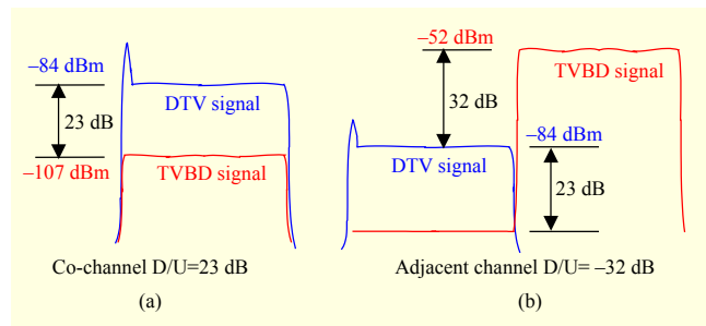
Fig. 4. (a) D/U ratio at grade B contour to protect DTV service from co-channel TVBD interference and (b) D/U ratio at grade B contour to protect DTV service from adjacent-channel TVBD interference.
