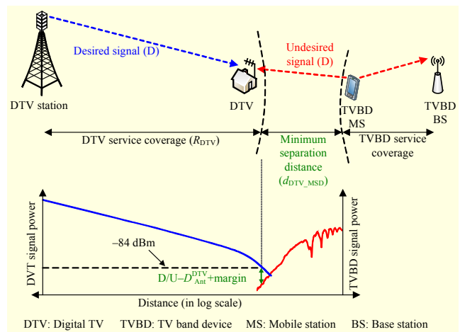
Fig. 1. Minimum separation distance of TVBD MS from edge of DTV service coverage (grade B contour).
