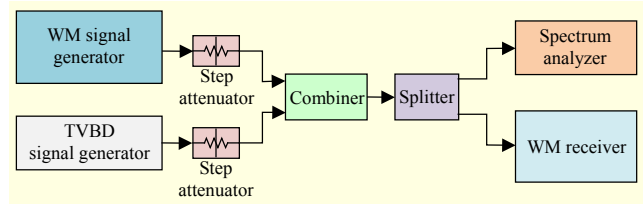
Fig. 5. Equipment setup to measure TOA and D/U for WM service.
