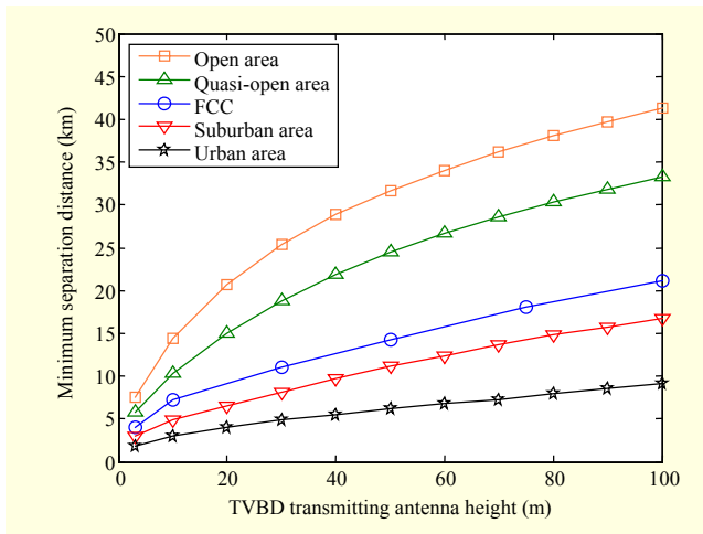
Fig. 8. Co-channel separation distances of 4 W fixed TVBDs from DTV protected contour for different ranges of TVBD transmit antenna heights in four geographic areas.
