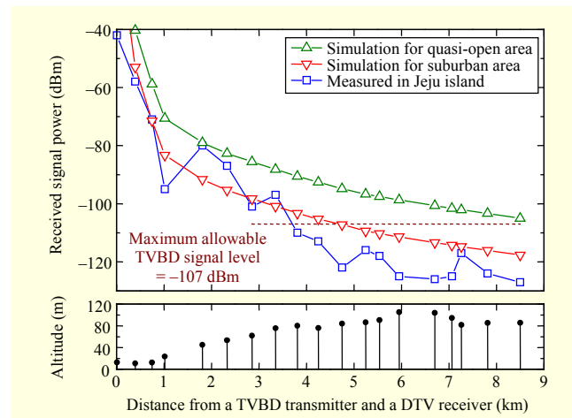
Fig. 12. Received interference signal power at ATSC DTV receiver with antenna height of 10 m; interference signal is transmitted from signal generator with transmitting antenna height of 10 m, which is located at distance ranging from 10 m to 8.5 km from DTV receiver.
