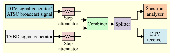
Fig. 3. Equipment setup to measure TOV and D/U for DTV service.
