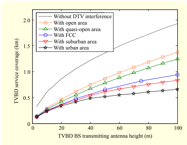
Fig. 10. Comparison of coverage reduction of TVBD network due to DTV interference with five different separation distances.
