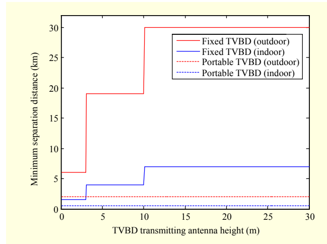
Fig. 7. Co-channel separation distance of TVBDs from noise-limited contour for both indoor and outdoor WM service.
