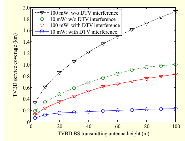
Fig. 9. Comparison of coverage reduction of TVBD network due to DTV interference with two different TVBD transmit power levels.
