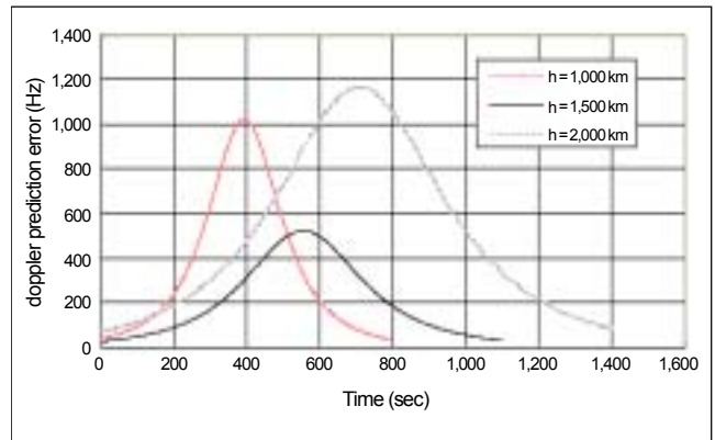
Fig. 4. Instantaneous error of the new prediction algorithm.
