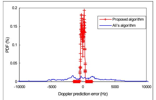
Fig. 2. Probability density function of the prediction error of the doppler frequency.
