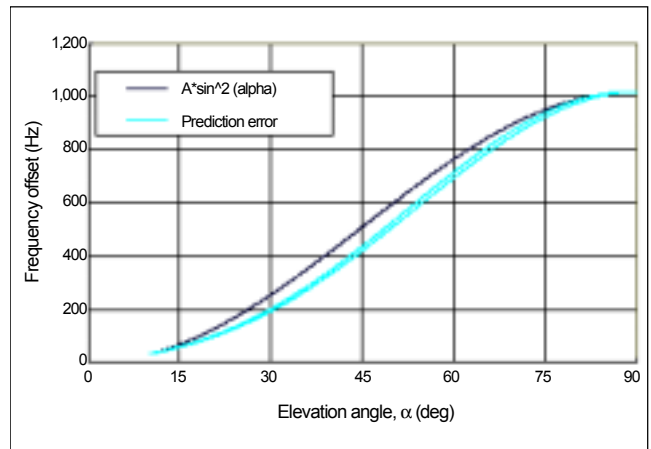
Fig. 5. Prediction error of doppler frequency shift versus the satellite elevation angle.
