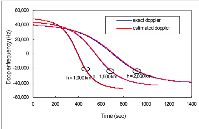
Fig. 3. Comparison between the exact Doppler frequency shift, f_D(t) and the predicted frequency shift, f_{DM1}(t) at f_c = 2.4 GHz.
