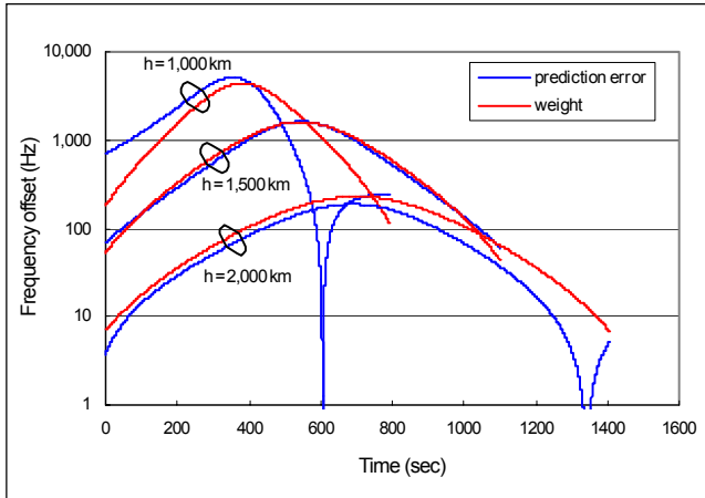
Fig. 6. Comparison between the prediction error and the weighting factor.
