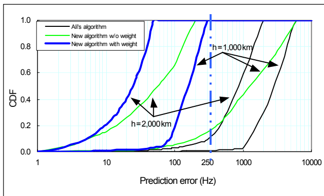
Fig. 8. Cumulative distribution function of the prediction error.
