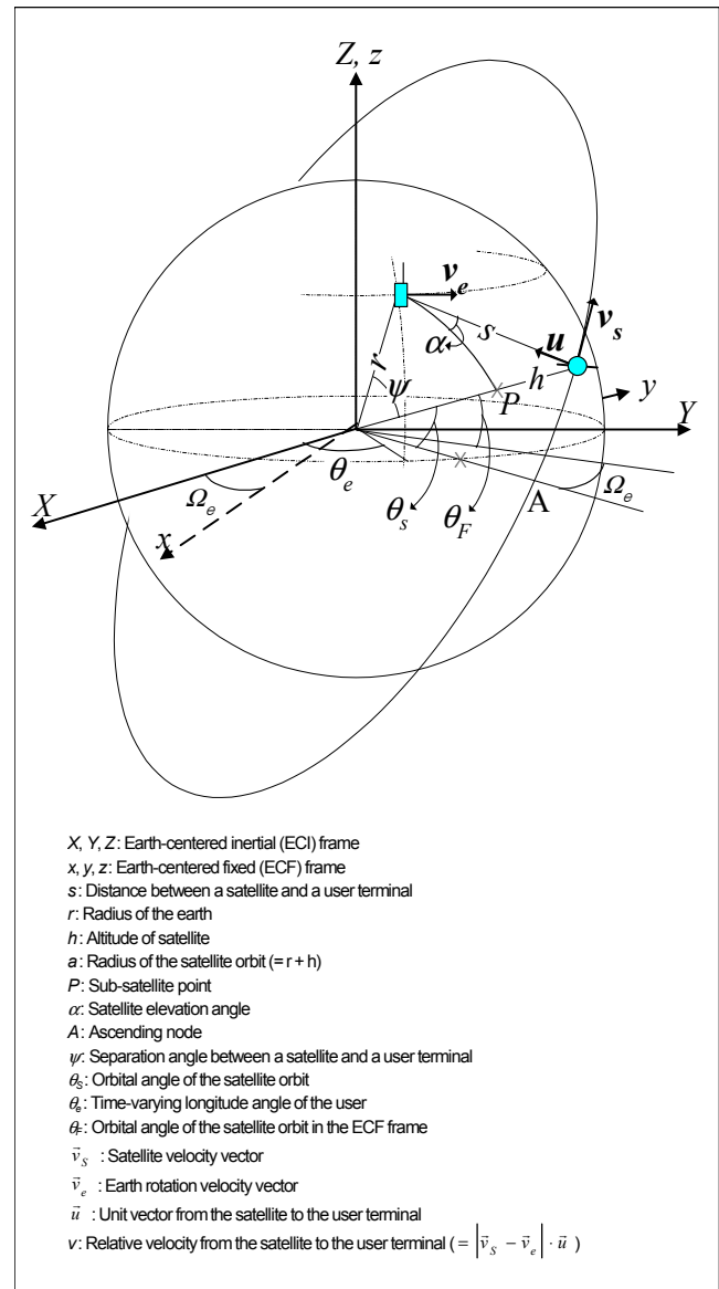
Fig. 1. Geographical configuration of the LEO satellite and the user terminal.
