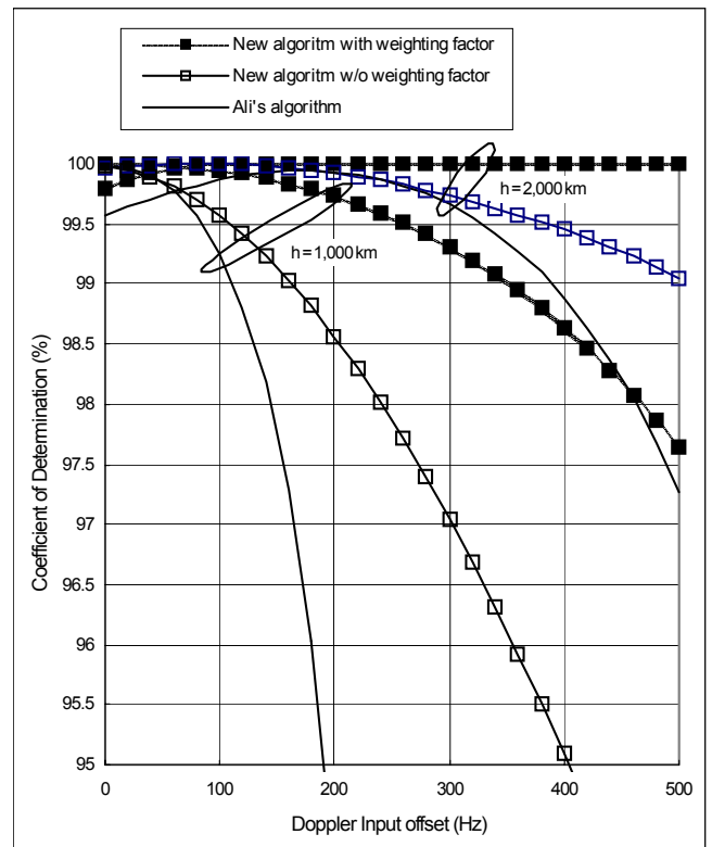
Fig. 7. Prediction accuracy comparison depending on doppler input offset.
