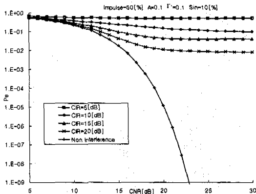
Fig. 9. Symbol error probabilities of 16QAM system (impulse=50%, sinusoidal=10%, rectangular=40%, A=0.1 , \Gamma'=0.1 ).
