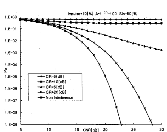
Fig. 7. Symbol error probabilities of 16QAM system (impulse=10 %, sinusoidal=50 %, rectangular=40 %, A=1, \Gamma'=100 ).
