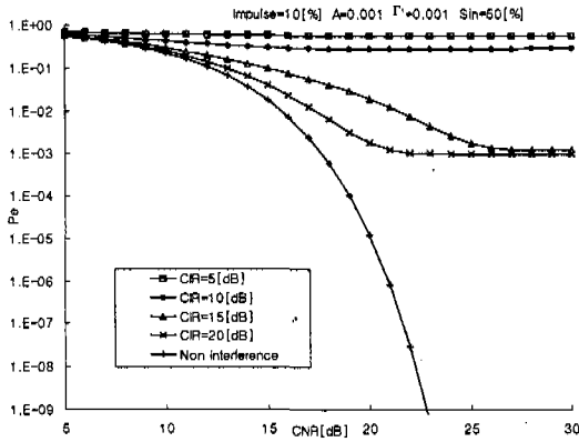
Fig. 5. Symbol error probabilities of 16QAM system (impulse=10 %, sinusoidal=50 %, rectangular=40 %, A=0.001, \Gamma'=0.001 ).
