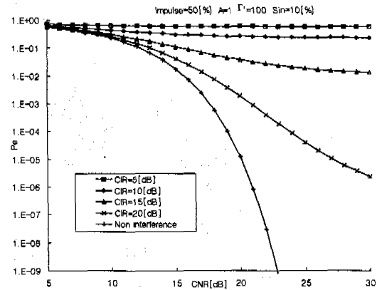
Fig. 10. Symbol error probabilities of 16QAM system (impulse=50%, sinusoidal=10%, rectangular=40%, A=1 , \Gamma'=100 ).
