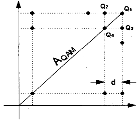
(a) Signal constellation for N-ary QAM signal.
