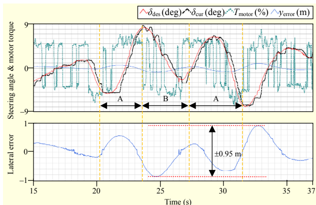
Fig. 20. Experimental results of double lane change for vehicle velocity of 100 kph and lane change section length of 100 m.
