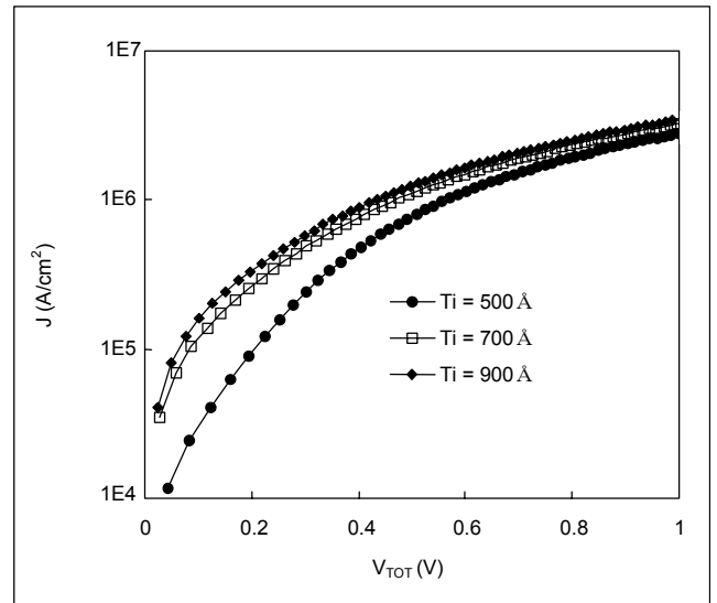
Fig. 1. I - V characteristic curve of the metal-semiconductor contact in a highly doped p+ junction. The contact hole size is 0.32 \mu\text{m} \times 0.32 \mu\text{m} . Closed circles, open squares, and closed diamonds represent data with Ti thicknesses of 500 \text{\AA} , 700 \text{\AA} , and 900 \text{\AA} , respectively.
