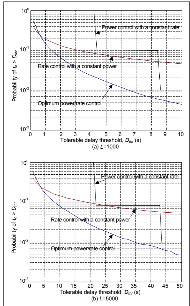
Fig. 3. Probabilities of instantaneous delay, t_d exceeding a tolerable threshold for three different control schemes with L=1000 and 5000 , P_0/N_f=50 dB, \sigma=12 , BPSK.
