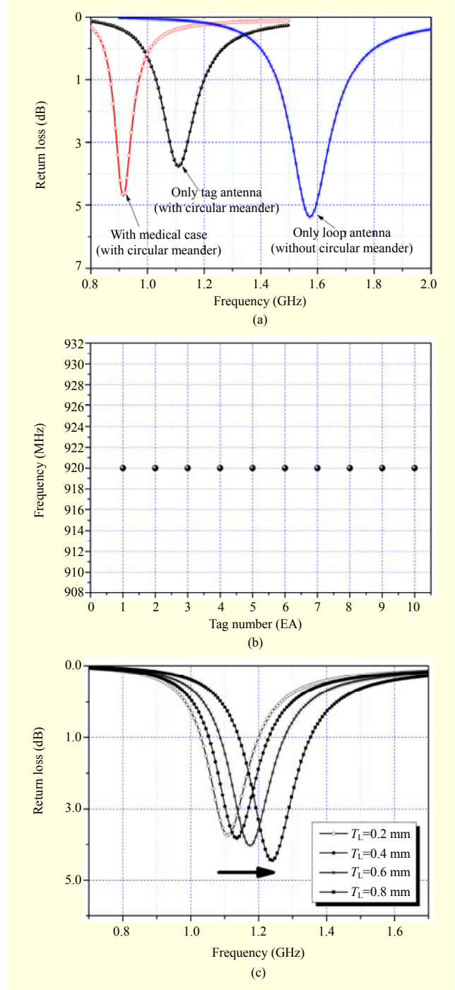
Fig. 2. (a) Simulated, (b) measured results of tag antenna, and (c) effects of different tag antenna values.
