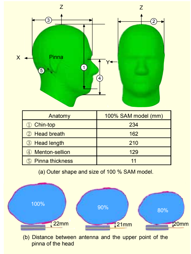
Fig. 2. Head models.
