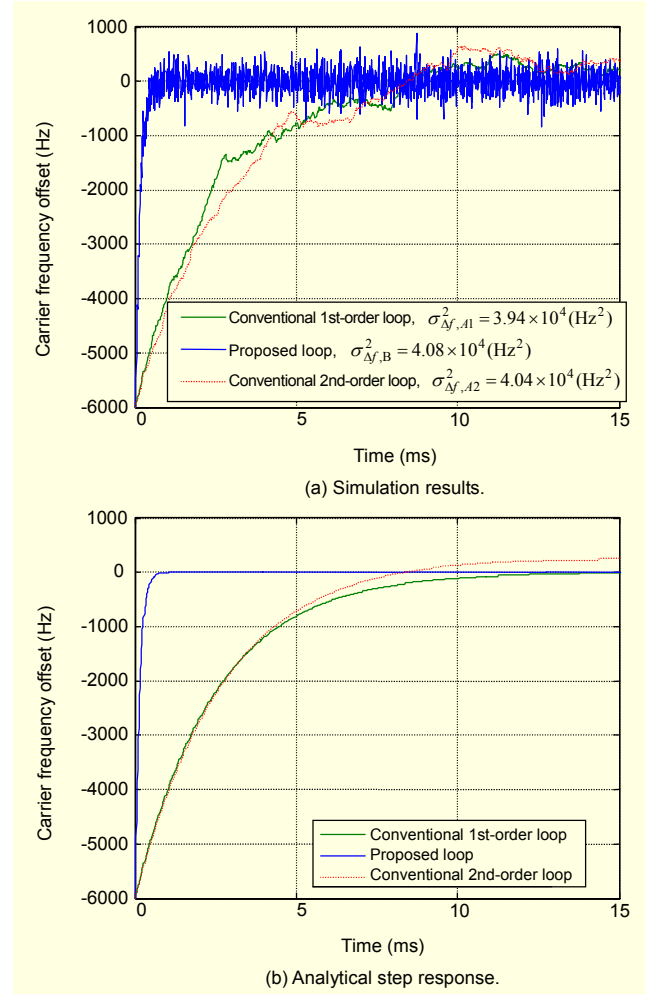
Fig. 3. Loop performances when the loops are designed for identical pull-in range of (-6.25, 6.25) kHz, equivalent noise bandwidth of 200 Hz, and steady-state jitter variance of 3.96 \times 10^4 \text{ Hz}^2 .
