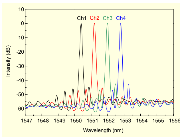
Fig. 4. Lasing spectra of the four channels measured at 60 mA.
