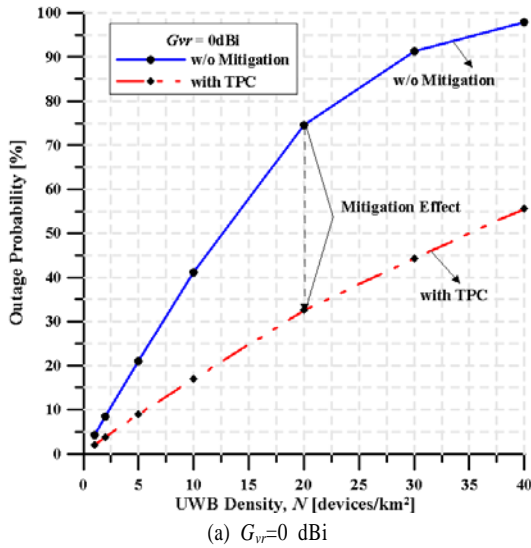
(a) G_{vr}=0 dBi
