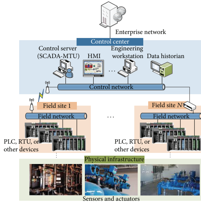
FIGURE 1: SCADA system general layout.
