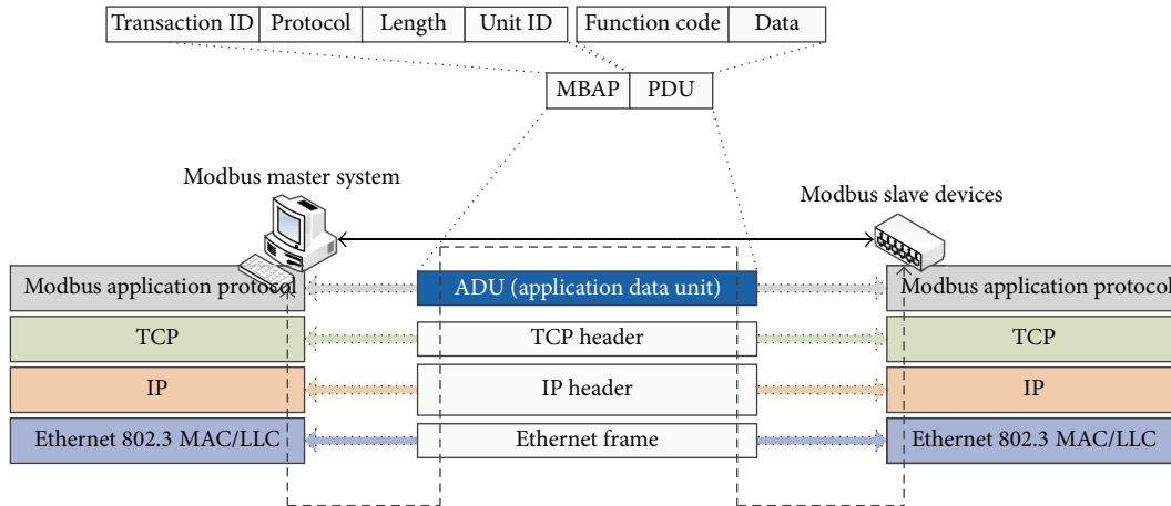
FIGURE 2: The format of Modbus TCP/IP ADU.
