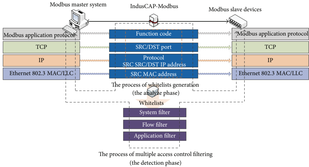
FIGURE 3: The packet processing flows of the IndusCAP-Gate system.
