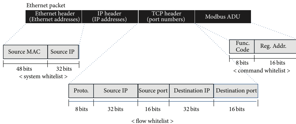
FIGURE 4: The format of whitelists.
