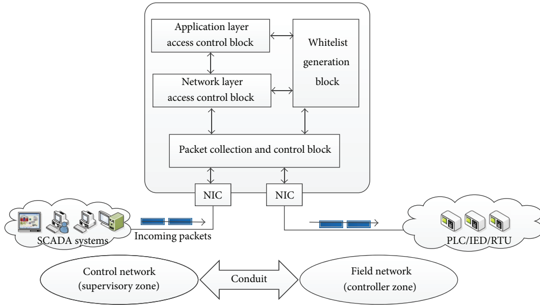
FIGURE 5: The system architecture.
