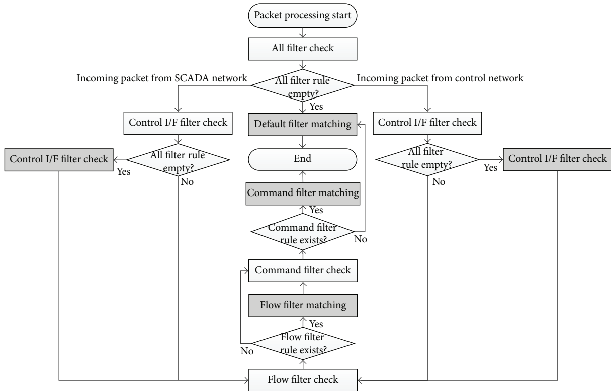
FIGURE 7: Overall packet processing flow through multiple access control filters.
