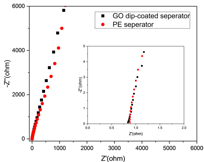
Figure 3. The Nyquist plot of 1 M LiPF 6 in EC/DMC using the GO dip-coated separator and the conventional separator, respectively.
