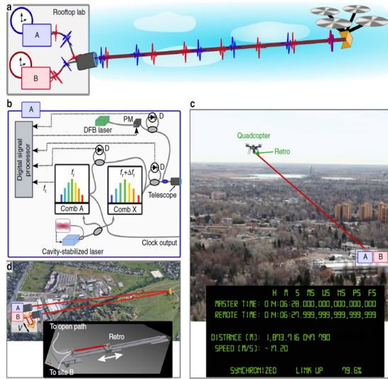
출처 H. Bergeron et al., "Femtosecond time synchronization of optical clocks off of a flying quadcopter," Nature Commun., 10, 1189, 2019. CC BY 4.0.
