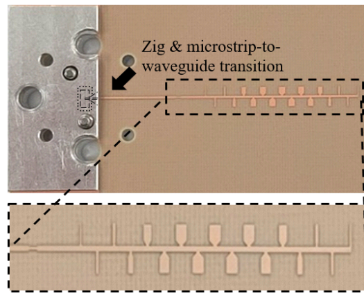
(a) 제안한 프로토타입 (a) Proposed prototype
