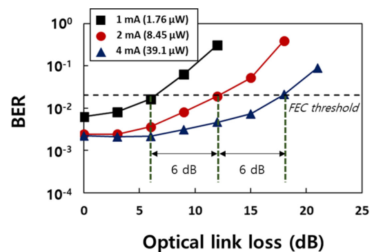
Fig. 7. Measured BER values as a function of the optical link loss for various photocurrents. The optical and wireless transmission distances were 10 km and \sim 3 cm, respectively. The carrier frequency was 300 GHz.
