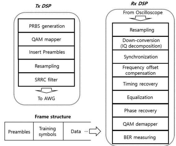
Fig. 4. DSP structures for sub-THz-band signal transmission.
