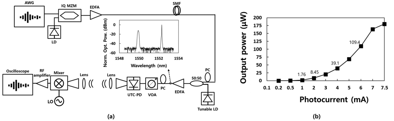
Fig. 3. (a) Experimental setup for downstream transmission. (b) Output power of the UTC-PD as a function of photocurrent and optical input power at a carrier frequency of 300 GHz.
