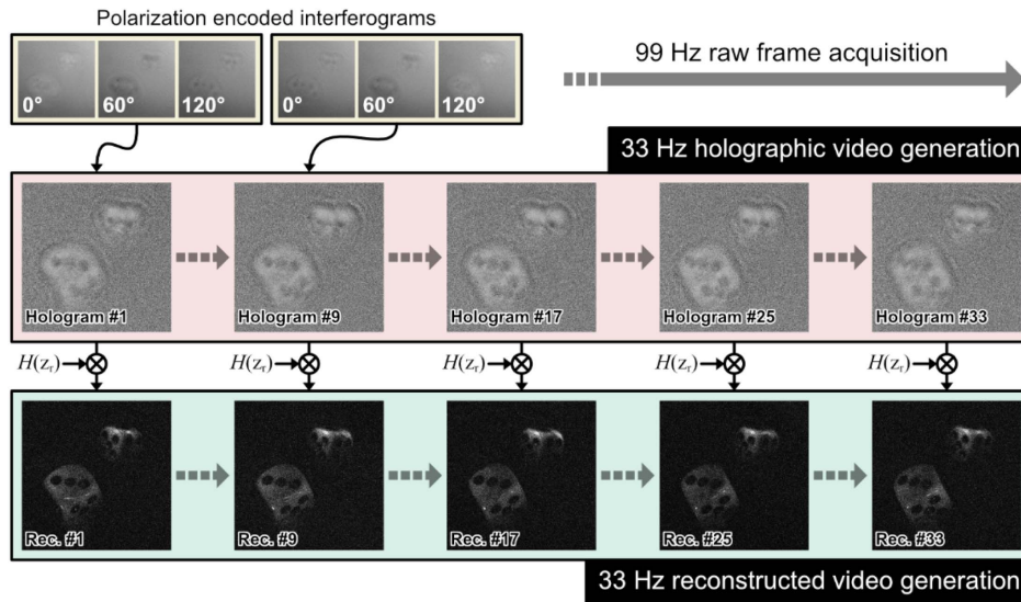
Fig. 7. Illustration of holographic video generation process from raw interferograms to reconstructed image. The holograms are obtained from the targets presented in Fig. 6. The rotation of Dice 1 is observed through frames. The holographic video, including the phase-angle data and reconstructed image at various depth planes, is available in Visualization 2. Rec., reconstructed image.
