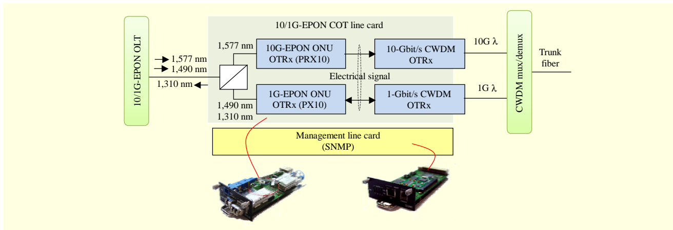
Fig. 3. Internal architecture of 10/1G-EPON COT line cards.
