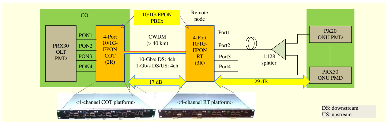
Fig. 2. 10/1G-EPON link structure using proposed hybrid-type PBEx.
