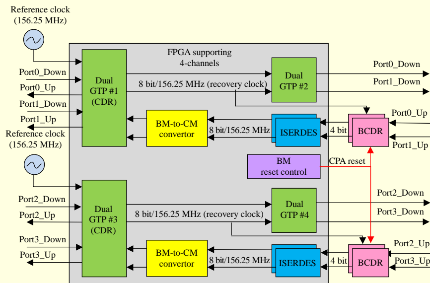
Fig. 5. Internal structure of FPGA for 3R-based signal regeneration [10].
