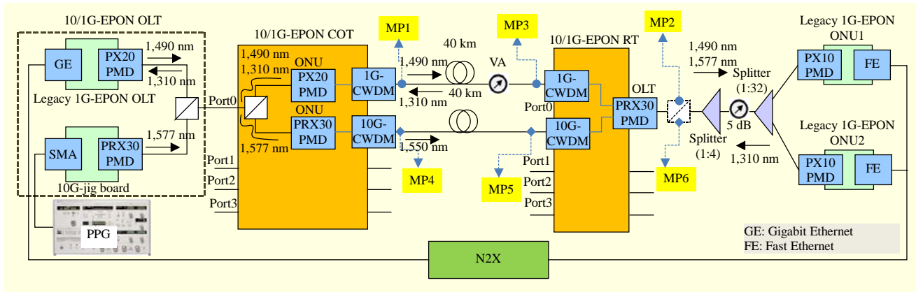
Fig. 6. Experimental setup for performance measurement of proposed hybrid-type 10/1G-EPON PBEx.
