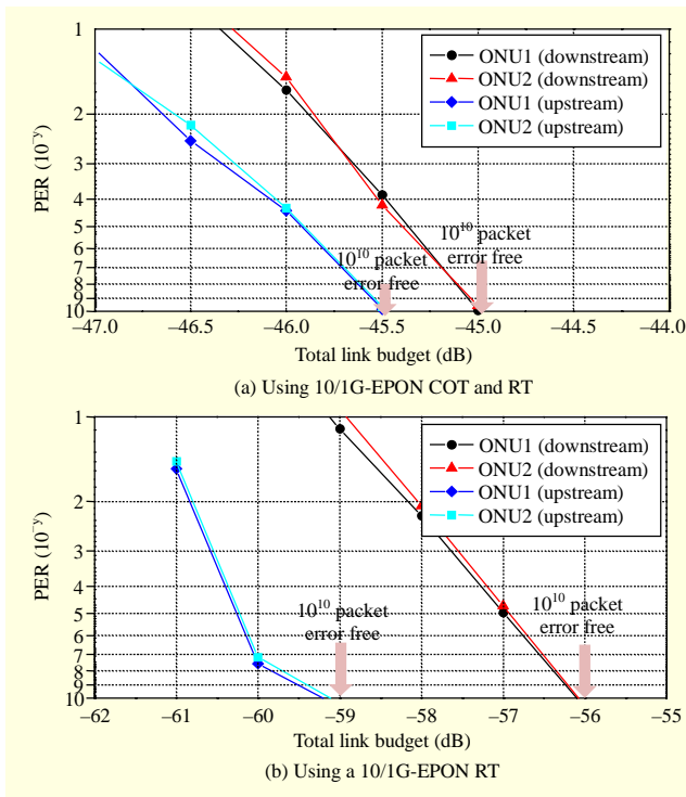
Fig. 9. PER results of 1.25-Gb/s EPON link.
