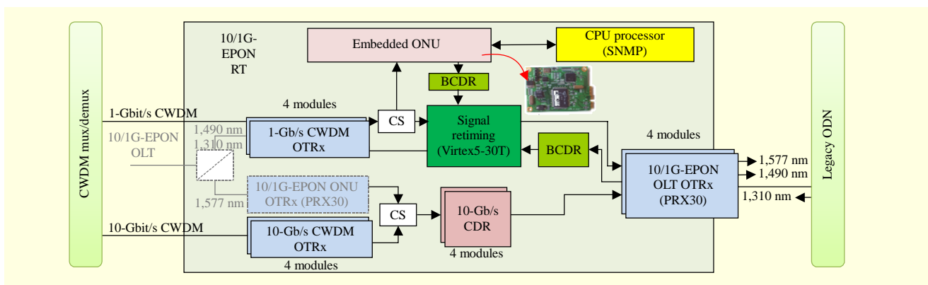
Fig. 4. Internal architecture of 10/1G-EPON RT.
