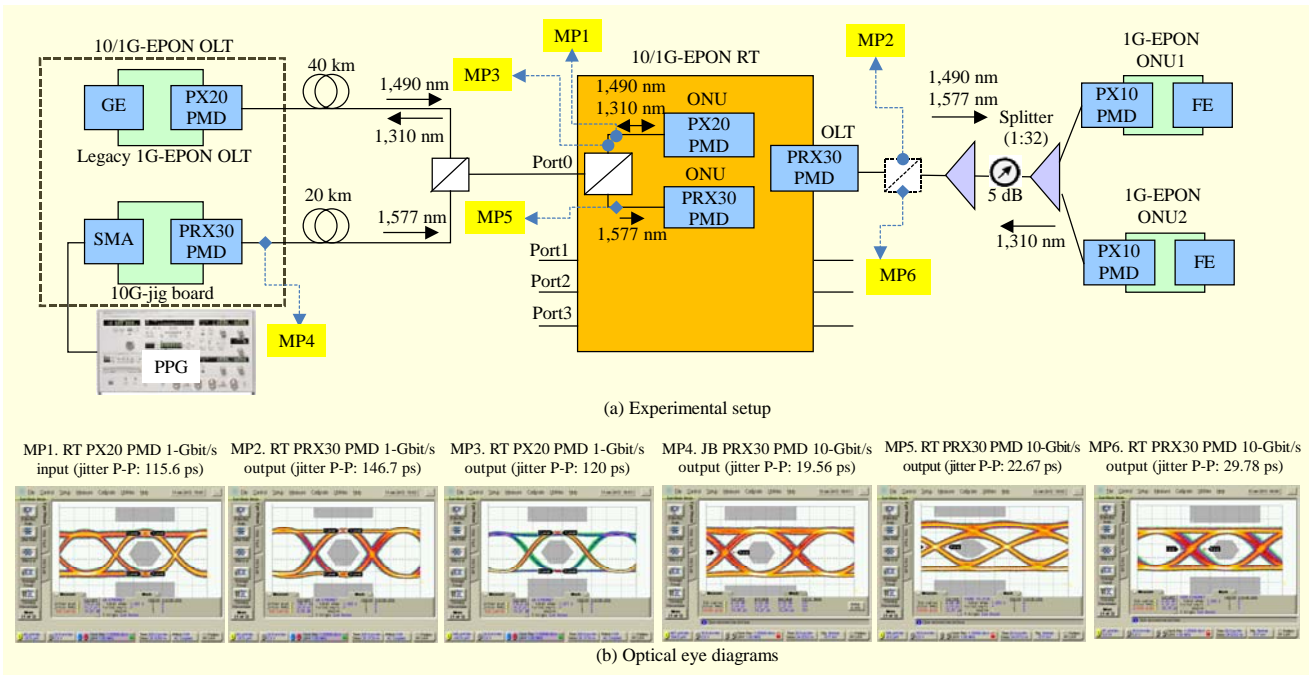
Fig. 8. Experimental setup and results at 10/1G-EPON RT.
