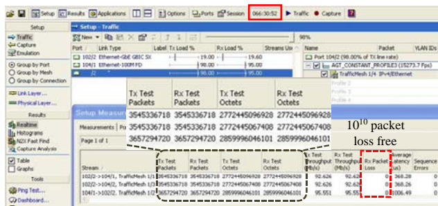
Fig. 10. Result of a long-term PER test.
