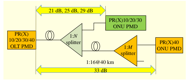
Fig. 1. 10G-EPON link structure suggested by IEEE 802.3 extended EPON study group [2], [3].
