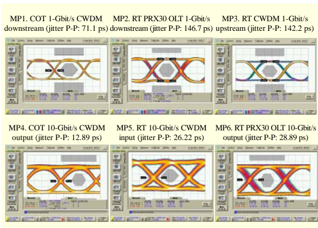
Fig. 7. Optical eye diagrams measured at each MP.
