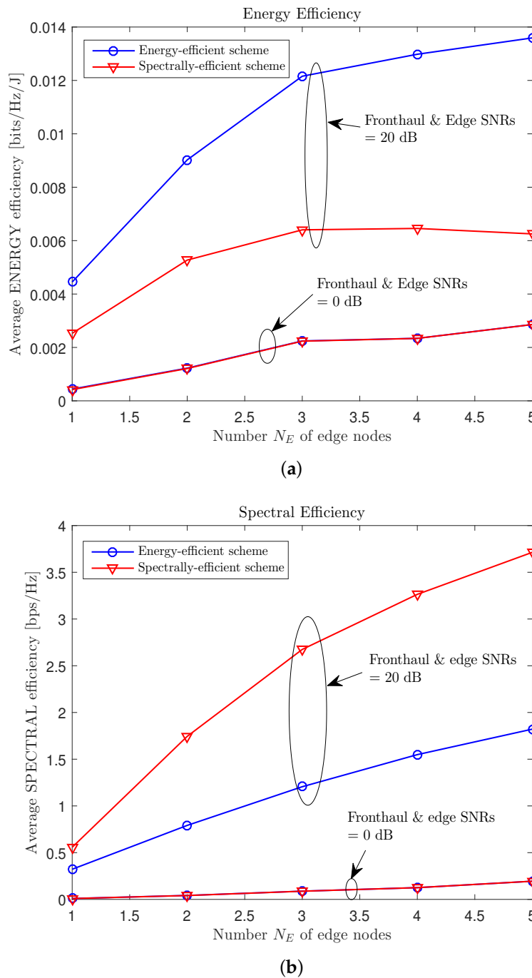
Figure 6. Average EE \Theta and SE R versus the number N_E of edge nodes with the “soft-transfer” fronthauling strategy (Section 3) for a cache-aided C-RAN system with n_C = 4 , N_U = 4 , n_{E,i} = 2 , n_{U,k} = 1 , \mu = 0.3 , and P_C/\sigma_E^2 = P_E/\sigma_U^2 \in \{0, 20\} dB ((a) EE; (b) SE).
